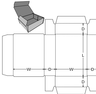
0. Standards\FEFCO Corrugated\0400 - Folder Type Boxes\FEFCO 0420 - Flanged Tuck Tray
