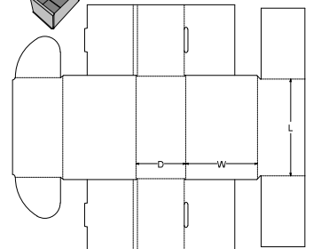
0. Standards\FEFCO Corrugated\0400 - Folder Type Boxes\FEFCO 0471 - Economy Tray RE Tuck Top CL
