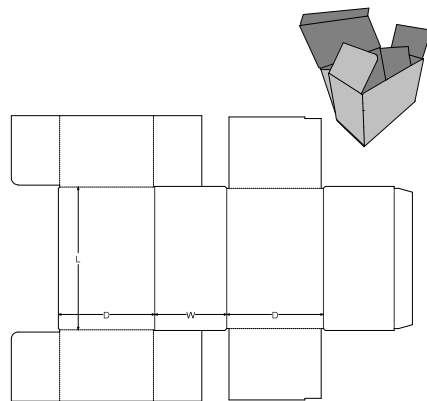
0. Standards\FEFCO Corrugated\0400 - Folder Type Boxes\FEFCO 0444 - Unglued Tuck To Back
