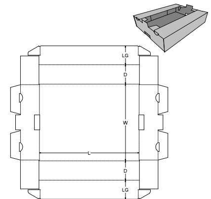
0. Standards\FEFCO Corrugated\0400 - Folder Type Boxes\FEFCO 0436 - Flanged Stacking Tray
