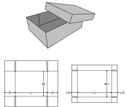
0. Standards\FEFCO Corrugated\0300 - Telescope Type Box\FEFCO 0306 - Side Slotted Tray with End Slotted Cover
