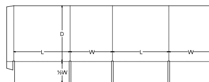
0. Standards\FEFCO Corrugated\0200 - Slotted Type Boxes\FEFCO 0200 EF - Half Slotted Container Extended Flaps - HSC EF
