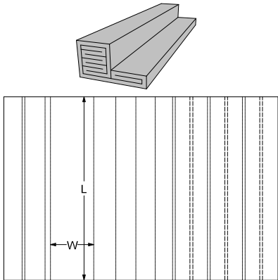
0. Standards\FEFCO Corrugated\0900 - Interior Fitments\FEFCO 0967 - Folded Edge Protector
