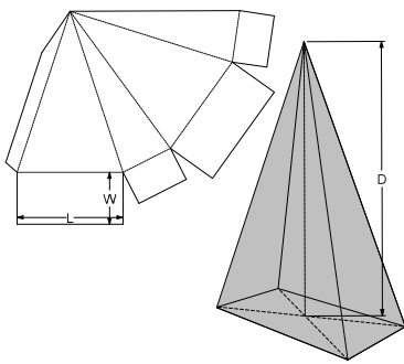
0. Standards\ECMA Folding Carton\Group C - Long Seam Glued, Non-Rect. Surface\ C30.20.10.01 - Rectangular Base Pyramid with Square Flaps C2210
