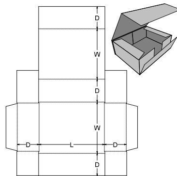
0. Standards\FEFCO Corrugated\0400 - Folder Type Boxes\FEFCO 0413 - Courier Pack, Diecut Side Taped
