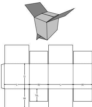
0. Standards\FEFCO Corrugated\0200 - Slotted Type Boxes\FEFCO 0206 - Overlap Sides, End Flaps Meet - SFF EFM
