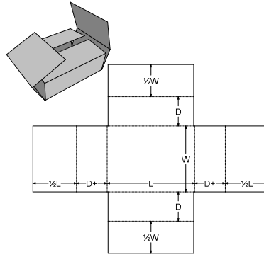
0. Standards\FEFCO Corrugated\0400 - Folder Type Boxes\FEFCO 0402 - One Piece Folder, All Panels Meet - OPF
