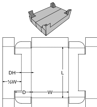
0. Standards\FEFCO Corrugated\0400 - Folder Type Boxes\FEFCO 0446 - Product Tray Stand Off Corners
