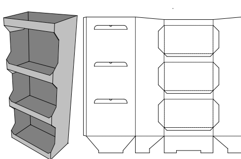
0. Standards\Display\2. Floor Standing Units\ Multi-Shelf Display - One Piece (2-4 Shelves) - Multi-Shelf Display - One Piece (2-4 Shelves) Weekender
