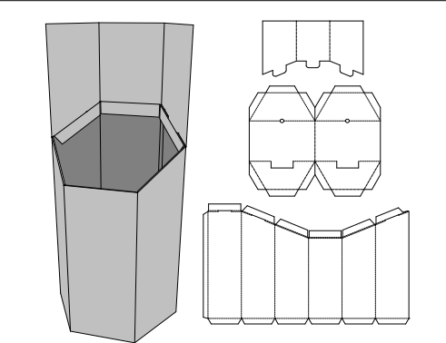
0. Standards\Display\2. Floor Standing Units\ Hexagonal Dumpbin (Sloping Front) - Standard hexagonal dumpbin with sloping front
