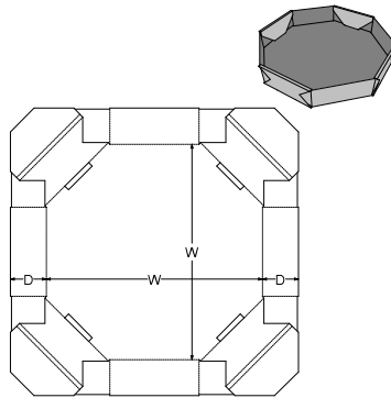
0. Standards\FEFCO Corrugated\0400 - Folder Type Boxes\FEFCO 0498 - Octagonal Rolled End Tray
