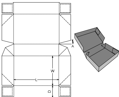
0. Standards\ECMA Folding Carton\Group B - Non-Long Seam Glued, Rect. Surface\B40.23.00.54 - Four Corner Hinged Lid with Webbed Corners B6121
