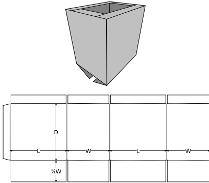
0. Standards\FEFCO Corrugated\0200 - Slotted Type Boxes\FEFCO 0209 - Flange Top, Regular Slotted Base - RSC
