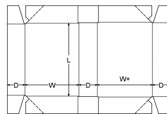
0. Standards\FEFCO Corrugated\0700 - Ready Glued - Self-Erecting Boxes\FEFCO 0759 - Style B - 4 Point Glued Tray with Lid
