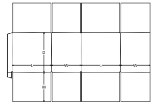
0. Standards\FEFCO Corrugated\0200 - Slotted Type Boxes\FEFCO 0203 EF - Full Overlap Slotted Container - EF
