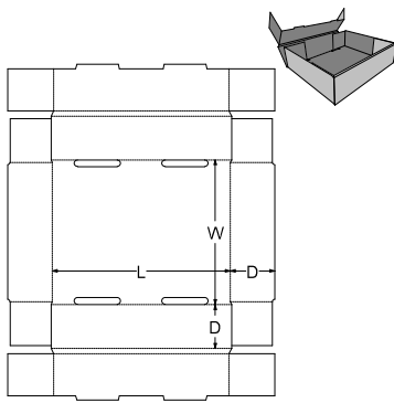
0. Standards\FEFCO Corrugated\0400 - Folder Type Boxes\FEFCO 0424 - Rolled Side Tray, Reinforced Ends
