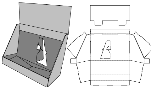
0. Standards\Display\1. Counter Top Units\Counterpack (Optional Slot On Header) - Standard Counterpack with optional slot on header
