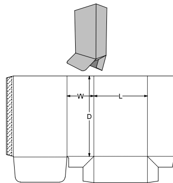
0. Standards\ECMA Folding Carton\Group A - Long Seam Glued, Rect. Surfaces\A45.01.01.00 - Open Top Sieve Proof Base A4501
