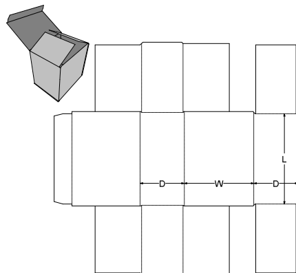
0. Standards\FEFCO Corrugated\0400 - Folder Type Boxes\FEFCO 0443 - Unglued Tuck To Front
