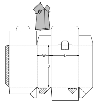
0. Standards\ECMA Folding Carton\Group A - Long Seam Glued, Rect. Surfaces\A61.20.01.03.31 (Securing Counterflap) - Double Tuck Full Crash Lock Base A6198
