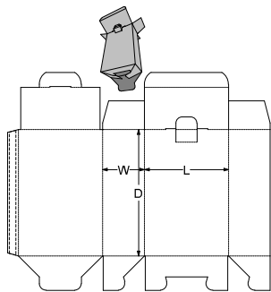
0. Standards\ECMA Folding Carton\Group A - Long Seam Glued, Rect. Surfaces\A55.20.01.03.31 (Securing Counterflap) - Double Tuck Snap Lock Base A5598
