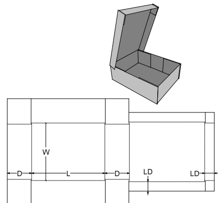
0. Standards\FEFCO Corrugated\0400 - Folder Type Boxes\FEFCO 0441 - Slitted Tray and Lid
