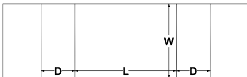
0. Standards\FEFCO Corrugated\0900 - Interior Fitments\FEFCO 0907 - Tube - Over End - Centre Gap
