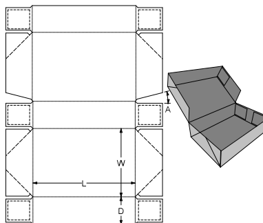
0. Standards\ECMA Folding Carton\Group B - Non-Long Seam Glued, Rect. Surface\B40.22.00.61 - 6 Corner Glued Tray with Hinged Lid B6020
