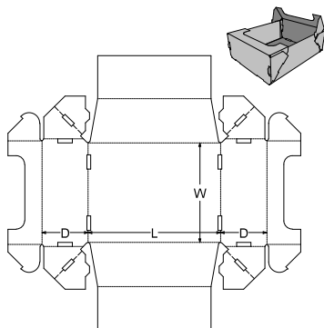
0. Standards\FEFCO Corrugated\0700 - Ready Glued - Self-Erecting Boxes\FEFCO 0774 - Flange Top Tray, Double Sides
