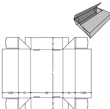
0. Standards\FEFCO Corrugated\0400 - Folder Type Boxes\FEFCO 0437 - End Lock Tray, Centre Joined
