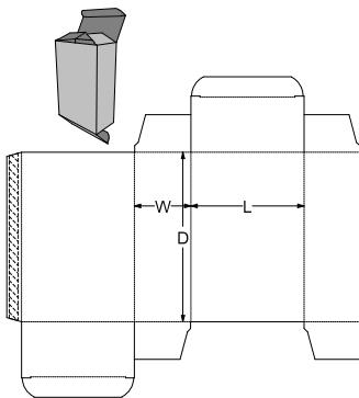
0. Standards\ECMA Folding Carton\Group A - Long Seam Glued, Rect. Surfaces\A20.20.01.03 - Inverted Reverse Tuck End A2220
