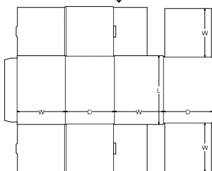
0. Standards\FEFCO Corrugated\0400 - Folder Type Boxes\FEFCO 0470 - Economy Tray RE Tuck Top
