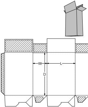
0. Standards\ECMA Folding Carton\Group A - Long Seam Glued, Rect. Surfaces\A60.11.00.03 - Standard Skillet Standard Crash Lock Base A6010
