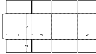
0. Standards\FEFCO Corrugated\0200 - Slotted Type Boxes\FEFCO 0205 - End Flaps Meet Slotted Container - CSO EFM
