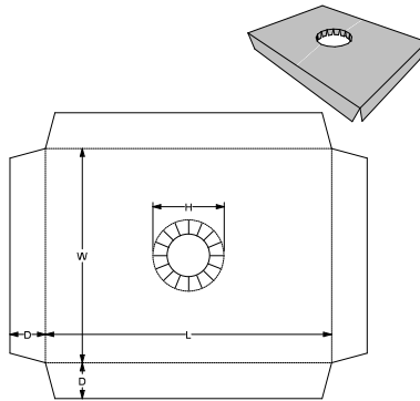
0. Standards\ECMA Folding Carton\Group F - Other Folding Carton Styles\F80.03.00.00 - 4 Sided Platform with Centre Hole F8003
