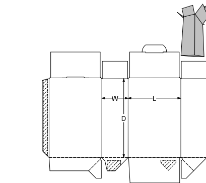
0. Standards\ECMA Folding Carton\Group A - Long Seam Glued, Rect. Surfaces\A61.56.01.03 - Edge Lock Skillet Full Crash Lock Base A6156
