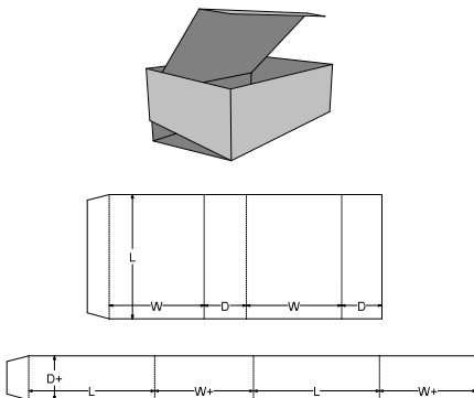
0. Standards\FEFCO Corrugated\0500 - Slide Type Boxes\FEFCO 0510 - Interlocking Sleeves Inner Tuck
