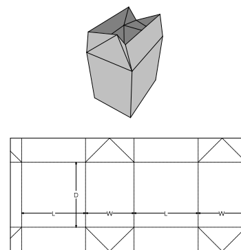
0. Standards\FEFCO Corrugated\0200 - Slotted Type Boxes\FEFCO 0226 - Bellows Style Container
