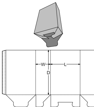
0. Standards\ECMA Folding Carton\Group A - Long Seam Glued, Rect. Surfaces\A55.01.01.00 - Open Ended Snap Lock Base A5501
