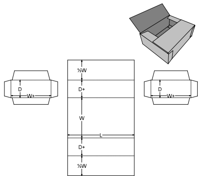
0. Standards\FEFCO Corrugated\0600 - Rigid Type Boxes - Bliss Boxes\FEFCO 0605 - Wrap with Part External End Caps
