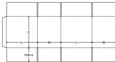
0. Standards\FEFCO Corrugated\0200 - Slotted Type Boxes\FEFCO 0202 - Overlap Slotted Container - POL
