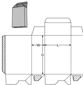
0. Standards\ECMA Folding Carton\Group A - Long Seam Glued, Rect. Surfaces\A60.20.00.03 - Tuck to Back Crash Lock Base A6020
