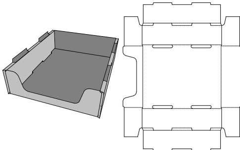
0. Standards\Display\3. Trays, Shelf Ready and Fillers\Stackable Rolled Side Tray - Stackable Rolled Side Tray (Fefco 0423)
