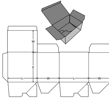
0. Standards\FEFCO Corrugated\0700 - Ready Glued - Self-Erecting Boxes\FEFCO 0713 - Crash Lock Base Auto Bottom, Tuck to Front Top - CLB/TF
