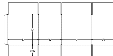
0. Standards\FEFCO Corrugated\0200 - Slotted Type Boxes\FEFCO 0201 - Regular Slotted Container - RSC
