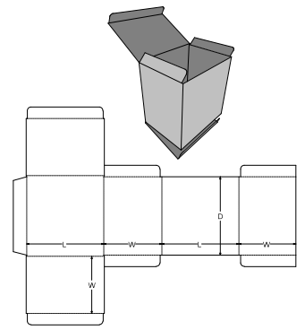
0. Standards\FEFCO Corrugated\0200 - Slotted Type Boxes\FEFCO 0210 - Aeroplane Tuck, Tuck to Front Container
