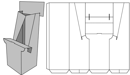
0. Standards\Display\2. Floor Standing Units\ Display Base - End Joint w/Flange - Display Base - End Joint w/Flange
