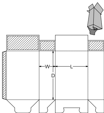
0. Standards\ECMA Folding Carton\Group A - Long Seam Glued, Rect. Surfaces\A55.11.01.03 - Square Flap Skillet Snap Lock Base A5510
