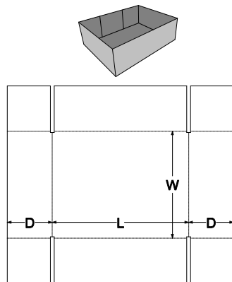
0. Standards\FEFCO Corrugated\0900 - Interior Fitments\FEFCO 0911 - Side Slotted Tray
