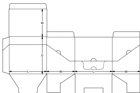
0. Standards\Display\3. Trays, Shelf Ready and Fillers\Shelf Ready Tuck to Front Top, Envelope Base - Shelf Ready Tuck to Front Top, Envelope Base (Fefco 0215)
