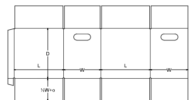
0. Standards\FEFCO Corrugated\0200 - Slotted Type Boxes\FEFCO 0202 EH - Overlap Slotted Container - EH
