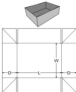
0. Standards\FEFCO Corrugated\0400 - Folder Type Boxes\FEFCO 0448 - Outfold Tray, Side Slots
