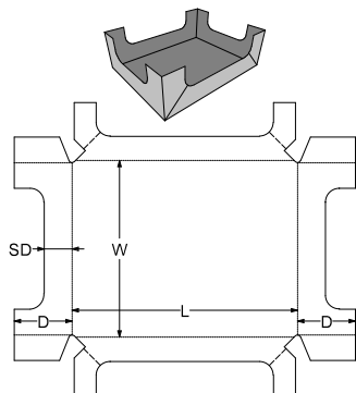
0. Standards\FEFCO Corrugated\0700 - Ready Glued - Self-Erecting Boxes\FEFCO 0770 - Style B - Open Sided Tray
