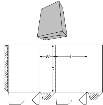
0. Standards\ECMA Folding Carton\Group A - Long Seam Glued, Rect. Surfaces\A60.01.00.00 - Open Ended Crash Lock Base A6001
