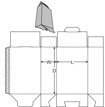
0. Standards\ECMA Folding Carton\Group A - Long Seam Glued, Rect. Surfaces\A55.56.01.03 - Edge Lock Skillet Snap Lock Base A5556
