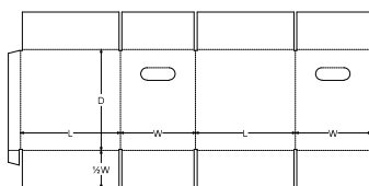
0. Standards\FEFCO Corrugated\0200 - Slotted Type Boxes\FEFCO 0201 EH - Regular Slotted Container Extended Glue Flap Hand Holes - RSC EH
