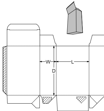
0. Standards\ECMA Folding Carton\Group A - Long Seam Glued, Rect. Surfaces\A61.20.01.01 - Tuck to Front Full Crash Lock Base A6120 Style B
