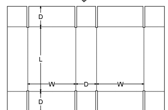
0. Standards\FEFCO Corrugated\0400 - Folder Type Boxes\FEFCO 0409 - Five Panel Folder, Side Taped - FPF
