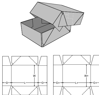
0. Standards\FEFCO Corrugated\0300 - Telescope Type Box\FEFCO 0304 - Infold Tray and Lid
