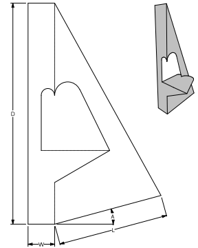
0. Standards\ECMA Folding Carton\Group F - Other Folding Carton Styles\F80.41.00.00 - Vertical Support Strut F8041
