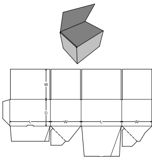
0. Standards\FEFCO Corrugated\0700 - Ready Glued - Self-Erecting Boxes\FEFCO 0703 - Style B - Full Crash Lock Auto Bottom, Full Overlapping Top - FCB/FOL
