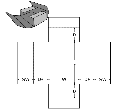
0. Standards\FEFCO Corrugated\0400 - Folder Type Boxes\FEFCO 0401 - One Piece Folder, Widths Meet - OPF
