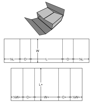
0. Standards\FEFCO Corrugated\0400 - Folder Type Boxes\FEFCO 0404 - 2 Piece Folder
