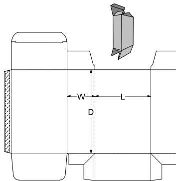
0. Standards\ECMA Folding Carton\Group A - Long Seam Glued, Rect. Surfaces\A45.20.01.01 - Tuck to Front Sieve Proof A4520 Style B
