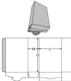
0. Standards\ECMA Folding Carton\Group A - Long Seam Glued, Rect. Surfaces\A10.01.01.00.38 (Reclosable opening w. Claw Lock) - Open Ended Locking Skillet A5601 Style A
