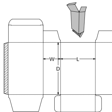
0. Standards\ECMA Folding Carton\Group A - Long Seam Glued, Rect. Surfaces\A40.20.03.01 - Tuck to Back Side Tuck A4020 Style A
