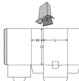
0. Standards\ECMA Folding Carton\Group A - Long Seam Glued, Rect. Surfaces\A20.01.03.00.31 (Securing Counterflap) - Open Top Double Tuck Base A9801
