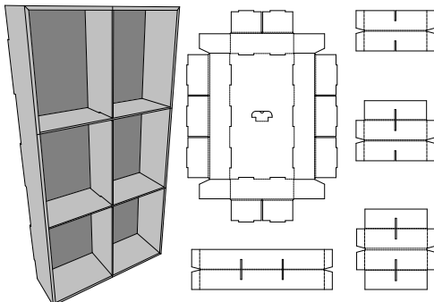
0. Standards\Display\3. Trays, Shelf Ready and Fillers\Multi-Cell Tray - Multi-Cell Tray
