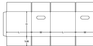
0. Standards\FEFCO Corrugated\0200 - Slotted Type Boxes\FEFCO 0201 HH - Regular Slotted Container Hand Holes - RSC HH
