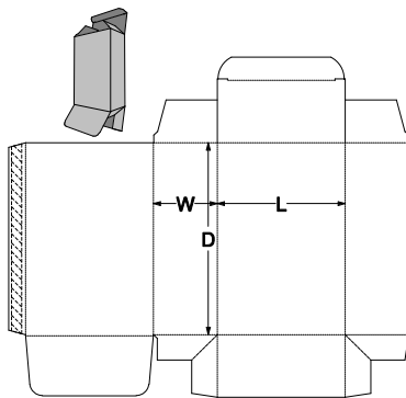
0. Standards\ECMA Folding Carton\Group A - Long Seam Glued, Rect. Surfaces\A45.20.01.03 - Tuck to Back Sieve Proof A4520 Style A
