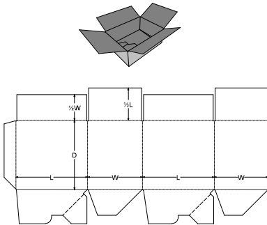
0. Standards\FEFCO Corrugated\0700 - Ready Glued - Self-Erecting Boxes\FEFCO 0712 - Crash Lock Base Auto Bottom, All Flaps Meet Top - CLB/AFM
