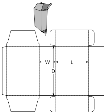
0. Standards\ECMA Folding Carton\Group A - Long Seam Glued, Rect. Surfaces\A40.40.03.03 - Side Tuck Top and Base A4040
