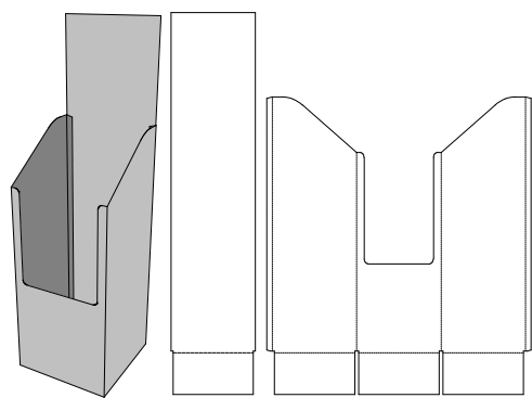
0. Standards\Display\2. Floor Standing Units\ Pallet Wrap - Turn Over Back w/Slotted Bottom - Pallet Wrap - Turn Over Back w/Slotted Bottom
