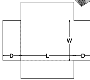
0. Standards\FEFCO Corrugated\0400 - Folder Type Boxes\FEFCO 0458 - Taped Tray
