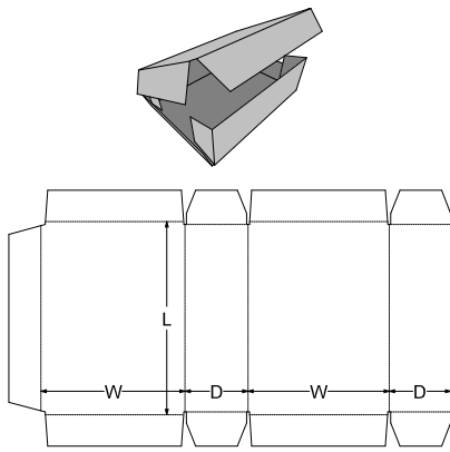
0. Standards\FEFCO Corrugated\0400 - Folder Type Boxes\FEFCO 0406 - Wrap Around Blank
