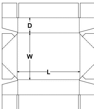
0. Standards\FEFCO Corrugated\0700 - Ready Glued - Self-Erecting Boxes\FEFCO 0718 - 4 Point Glued Tray
