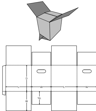
0. Standards\FEFCO Corrugated\0200 - Slotted Type Boxes\FEFCO 0206 EH - Overlap Sides, End Flaps Meet - SFF EFM EH
