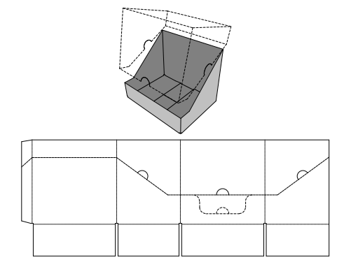
0. Standards\Display\3. Trays, Shelf Ready and Fillers\Shelf Ready Half Slotted Container - Shelf Ready Half Slotted Container (Fefco 0200)
