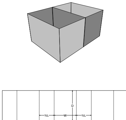
0. Standards\FEFCO Corrugated\0900 - Interior Fitments\FEFCO 0921 - Interior Buffer
