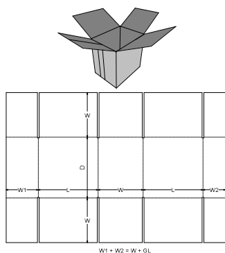
0. Standards\FEFCO Corrugated\0200 - Slotted Type Boxes\FEFCO 0231 - Full Overlapping Container, Centre Seam on Ends
