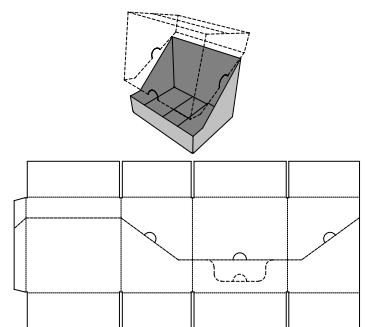
0. Standards\Display\3. Trays, Shelf Ready and Fillers\Shelf Ready Regular Slotted Container - Shelf Ready Regular Slotted Container (Fefco 0201)
