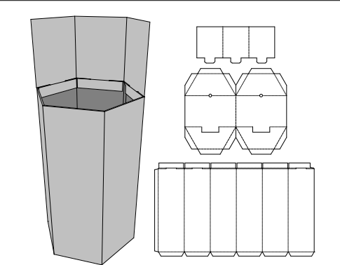
0. Standards\Display\2. Floor Standing Units\ Hexagonal Dumpbin - Standard hexagonal dumpbin
