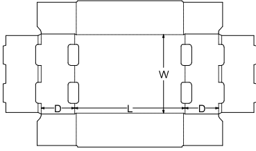
0. Standards\FEFCO Corrugated\0400 - Folder Type Boxes\FEFCO 0435 - Rolled End Stacking Tray
