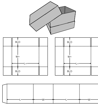
0. Standards\FEFCO Corrugated\0300 - Telescope Type Box\FEFCO 0310 - Sleeve with Slotted Tray and End to End Lid
