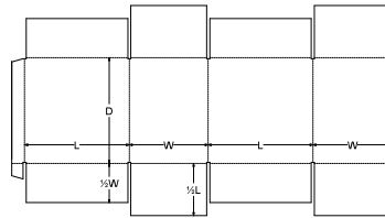
0. Standards\FEFCO Corrugated\0200 - Slotted Type Boxes\FEFCO 0204 EF - All Flaps Meet Slotted Container - AFM - CSSC EF
