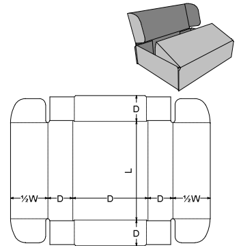
0. Standards\FEFCO Corrugated\0400 - Folder Type Boxes\FEFCO 0416 - One Piece Folder, Centre Tuck - OPF
