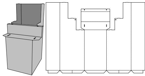
0. Standards\Display\2. Floor Standing Units\ Display StepBase - Centre Joint - Display StepBase - Centre Joint
