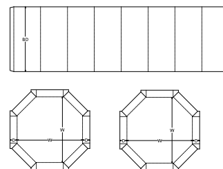
0. Standards\FEFCO Corrugated\0300 - Telescope Type Box\FEFCO 0350 - Octagonal Bulk Box - Glued Ends
