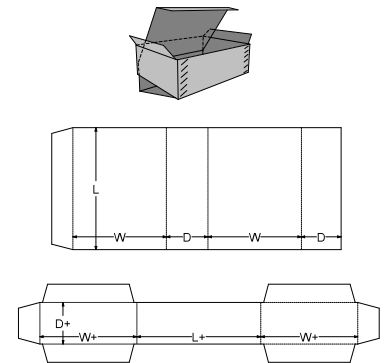
0. Standards\FEFCO Corrugated\0500 - Slide Type Boxes\FEFCO 0511 - Interlocking Sleeves Inner Tuck with Dust Flaps
