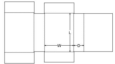
0. Standards\FEFCO Corrugated\0400 - Folder Type Boxes\FEFCO 0497 - 5 Panel Folder - Non-Glued
