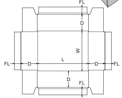
0. Standards\FEFCO Corrugated\0400 - Folder Type Boxes\FEFCO 0430 - Roll Over Top Tray
