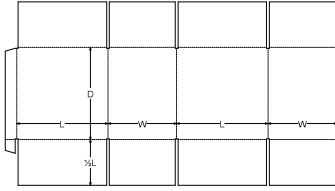
0. Standards\FEFCO Corrugated\0200 - Slotted Type Boxes\FEFCO 0205 EF - End Flaps Meet Slotted Container - CSO EFM EF
