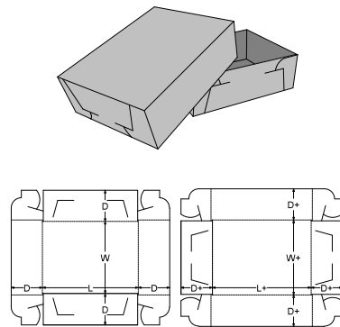
0. Standards\FEFCO Corrugated\0300 - Telescope Type Box\FEFCO 0307 - Self Locking Tray and Lid
