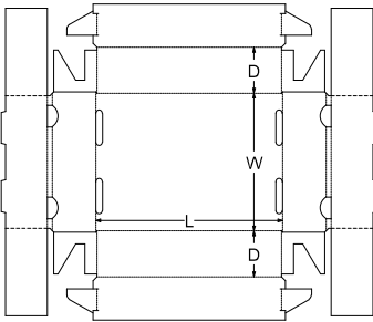
0. Standards\FEFCO Corrugated\0400 - Folder Type Boxes\FEFCO 0432 - Locking Flanged Tray
