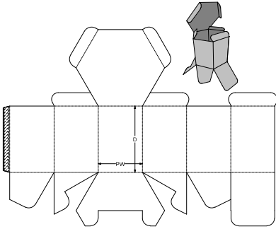
0. Standards\ECMA Folding Carton\Group C - Long Seam Glued, Non-Rect. Surface\ C10.40.55.20 - Hexagonal Snap Lock Base C4055
