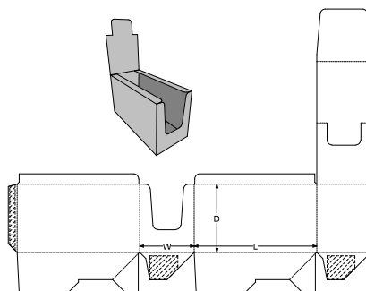
0. Standards\ECMA Folding Carton\Group A - Long Seam Glued, Rect. Surfaces\A60.20.00.04.35 (Display Outer) - Display Outer Crash Lock Base FC0602
