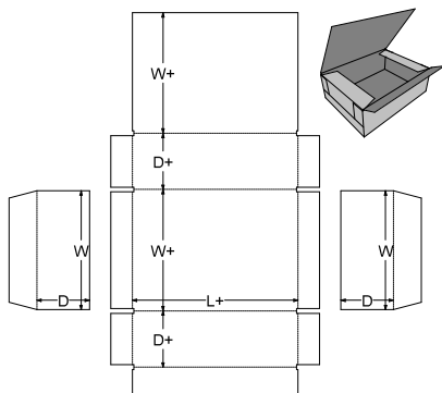
0. Standards\FEFCO Corrugated\0600 - Rigid Type Boxes - Bliss Boxes\FEFCO 0601 - Bliss Box with End Flaps
