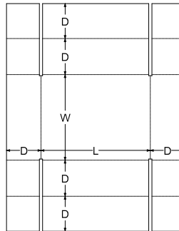
0. Standards\FEFCO Corrugated\0400 - Folder Type Boxes\FEFCO 0455 - Tray Folded Sides
