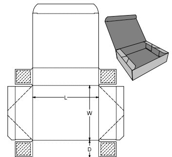
0. Standards\ECMA Folding Carton\Group B - Non-Long Seam Glued, Rect. Surface\B40.22.00.50 - Four Corner Hinged Lid B4050
