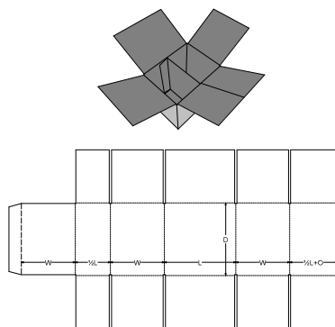
0. Standards\FEFCO Corrugated\0200 - Slotted Type Boxes\FEFCO 0228 - Full Overlapping Container, Centre Seam, Centre Divider
