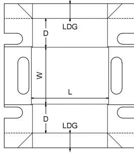
0. Standards\FEFCO Corrugated\0400 - Folder Type Boxes\FEFCO 0434 - Flanged Produce Tray
