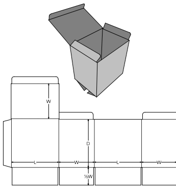
0. Standards\FEFCO Corrugated\0200 - Slotted Type Boxes\FEFCO 0212 - Tuck to Front Top, Regular Slotted Base - RSC
