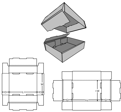
0. Standards\FEFCO Corrugated\0300 - Telescope Type Box\FEFCO 0330 - Rolled Side Tray & Push On Rolled End Tray
