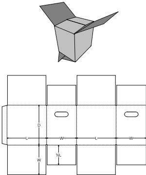
0. Standards\FEFCO Corrugated\0200 - Slotted Type Boxes\FEFCO 0206 HH - Overlap Sides, End Flaps Meet - SFF EFM
