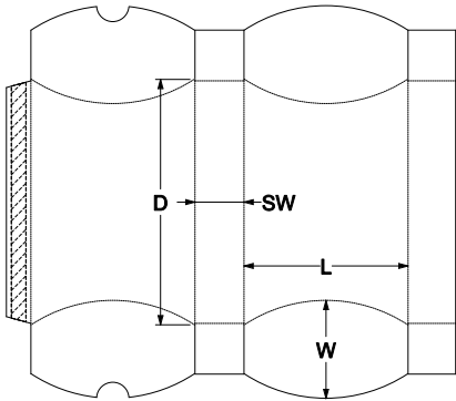
0. Standards\ECMA Folding Carton\Group F - Other Folding Carton Styles\F70.01.00.00 Style B - Pillow Pack Side Walls F7001 Style B
