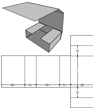
0. Standards\FEFCO Corrugated\0400 - Folder Type Boxes\FEFCO 0400 - One Piece Folder, Wrap Around - OPF
