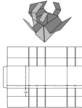
0. Standards\FEFCO Corrugated\0200 - Slotted Type Boxes\FEFCO 0208 - Slotted Containers with Holders
