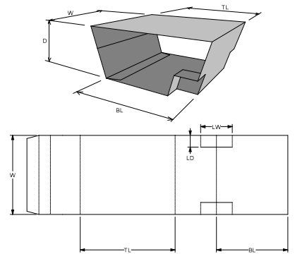
0. Standards\ECMA Folding Carton\Group E - Product Related or Integrated\E31.20.00.00 Style B - Angled Glued Sleeve E3120 Style B
