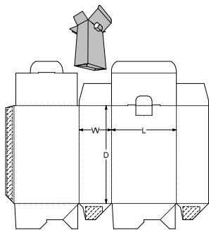
0. Standards\ECMA Folding Carton\Group A - Long Seam Glued, Rect. Surfaces\A60.20.00.03.31 (Securing Counterflap) - FC0110 - Double Tuck Crash Lock Base
