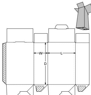
0. Standards\ECMA Folding Carton\Group A - Long Seam Glued, Rect. Surfaces\A60.56.00.03 - Edge Lock Skillet Crash Lock Base A6056
