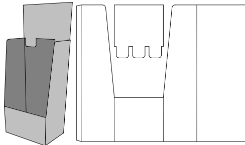
0. Standards\Display\2. Floor Standing Units\ Casewrap Display - Casewrap Display with Header
