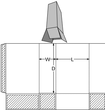
0. Standards\ECMA Folding Carton\Group A - Long Seam Glued, Rect. Surfaces\A10.01.03.00 - Open Ended Full Overlap Skillet A1001
