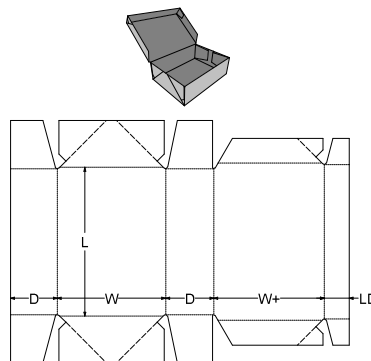
0. Standards\FEFCO Corrugated\0700 - Ready Glued - Self-Erecting Boxes\FEFCO 0761 - Style B - 6 Point Glued Tray with Cover
