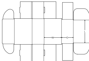
0. Standards\FEFCO Corrugated\0400 - Folder Type Boxes\FEFCO 0472 - Economy Tray RE Double Tuck Top CL
