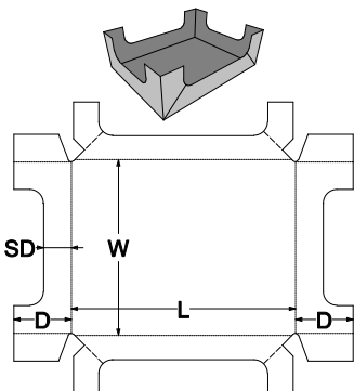
0. Standards\FEFCO Corrugated\0700 - Ready Glued - Self-Erecting Boxes\FEFCO 0770 - Open Sided Tray
