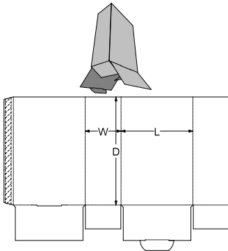
0. Standards\ECMA Folding Carton\Group A - Long Seam Glued, Rect. Surfaces\A56.01.03.00 - Open Top Edge Lock Skillet A5601 Style B
