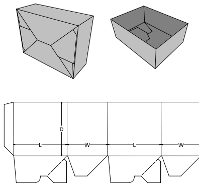
0. Standards\FEFCO Corrugated\0700 - Ready Glued - Self-Erecting Boxes\FEFCO 0700 - Style B - Crash Lock Auto Bottom, Open Top - CLB/OT
