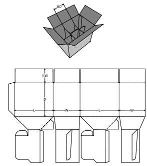
0. Standards\FEFCO Corrugated\0700 - Ready Glued - Self-Erecting Boxes\FEFCO 0715 - Crash Lock Base Auto Bottom with Divider, Regular Slotted Top - CLB/RSC
