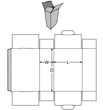
0. Standards\ECMA Folding Carton\Group A - Long Seam Glued, Rect. Surfaces\A56.56.03.03 - Edge Lock Skillet A5656
