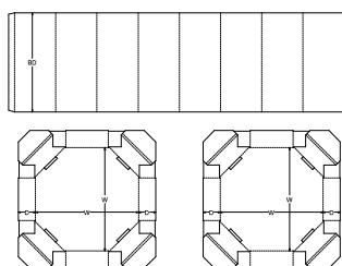
0. Standards\FEFCO Corrugated\0300 - Telescope Type Box\FEFCO 0351 - Octagonal Bulk Box - Rolled Ends
