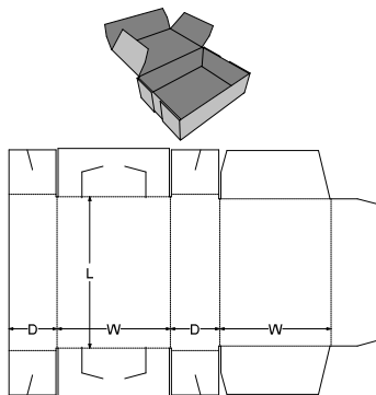
0. Standards\FEFCO Corrugated\0400 - Folder Type Boxes\FEFCO 0442 - End Slit Lock Tuck Tray
