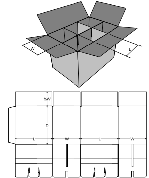
0. Standards\FEFCO Corrugated\0200 - Slotted Type Boxes\FEFCO 0207 - Slotted Container with Dividers - RSC
