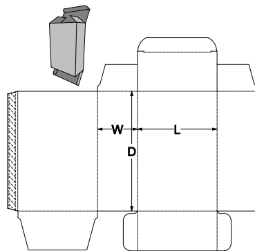
0. Standards\ECMA Folding Carton\Group A - Long Seam Glued, Rect. Surfaces\A40.20.03.03 - Tuck to Front Side Tuck A4020 Style B
