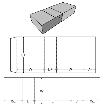
0. Standards\FEFCO Corrugated\0500 - Slide Type Boxes\FEFCO 0509 - Interlocking Sleeves Inner Centre Join
