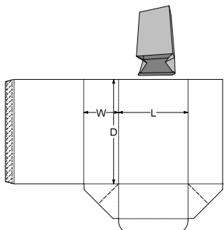
0. Standards\ECMA Folding Carton\Group A - Long Seam Glued, Rect. Surfaces\A20.01.03.00.99 (Webbed Tuck) - Open Top Webbed Tuck Base A9901
