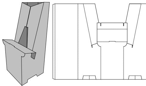
0. Standards\Display\2. Floor Standing Units\ Display Base - End Joint (2) - Display Base - End Joint (2)
