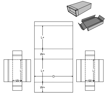
0. Standards\FEFCO Corrugated\0600 - Rigid Type Boxes - Bliss Boxes\FEFCO 0615 - Wrap with Full Cover Buffer End Caps
