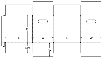
0. Standards\FEFCO Corrugated\0200 - Slotted Type Boxes\FEFCO 0204 EH - All Flaps Meet Slotted Container - AFM - CSSC EH
