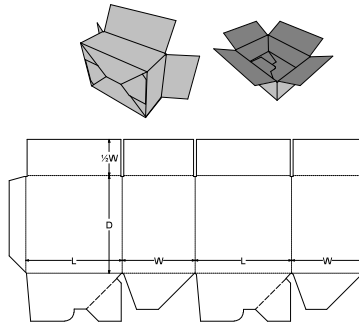
0. Standards\FEFCO Corrugated\0700 - Ready Glued - Self-Erecting Boxes\FEFCO 0711 - Style B - Crash Lock Auto Bottom, Regular Slotted Top - CLB/RSC
