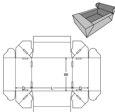
0. Standards\FEFCO Corrugated\0700 - Ready Glued - Self-Erecting Boxes\FEFCO 0773 - Flange Top Tray
