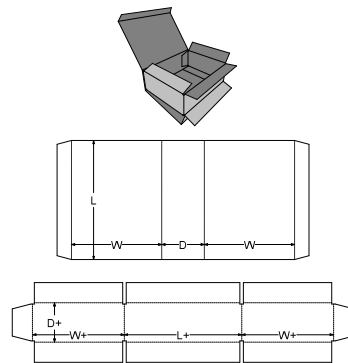
0. Standards\FEFCO Corrugated\0500 - Slide Type Boxes\FEFCO 0512 - Interlocking Sleeves Side Glued
