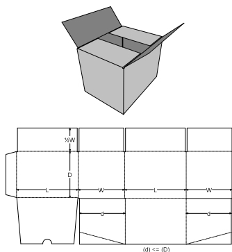
0. Standards\FEFCO Corrugated\0200 - Slotted Type Boxes\FEFCO 0225 - File Base Slotted Container - RSC
