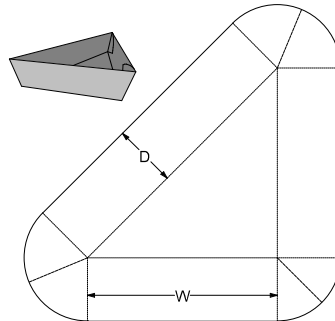
0. Standards\ECMA Folding Carton\Group D - Non-Long Seam Glued, Non-Rect. Surface\ D10.10.11.00 - Triangular Single-Walled Carton with Dust-Proof Corners D1011
