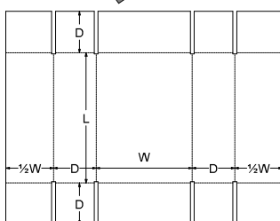
0. Standards\FEFCO Corrugated\0400 - Folder Type Boxes\FEFCO 0411 - Five Panel Folder, Centre Seam - FPF
