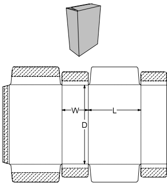
0. Standards\ECMA Folding Carton\Group A - Long Seam Glued, Rect. Surfaces\A11.11.03.03 (Skillet) - Overlapping Skillet
