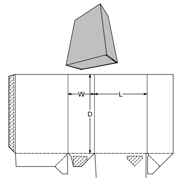
0. Standards\ECMA Folding Carton\Group A - Long Seam Glued, Rect. Surfaces\A61.01.01.00 - Open Ended Full Crash Lock Base A6101
