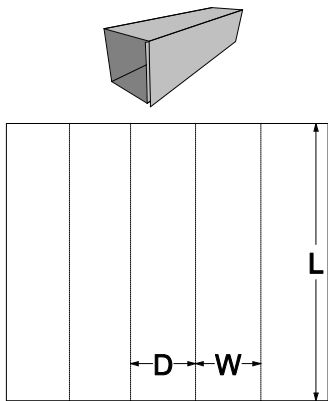
0. Standards\FEFCO Corrugated\0900 - Interior Fitments\FEFCO 0914 - Tube - 5 Panel
