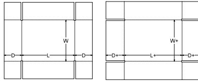
0. Standards\FEFCO Corrugated\0300 - Telescope Type Box\FEFCO 0301 - Side Slotted Tray with End Slotted Lid
