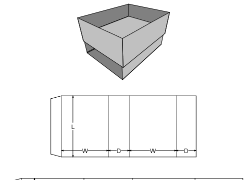
0. Standards\FEFCO Corrugated\0500 - Slide Type Boxes\FEFCO 0507 - Interlocking Sleeves C
