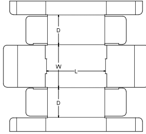
0. Standards\FEFCO Corrugated\0400 - Folder Type Boxes\FEFCO 0431 - Reinforced Flanged Tray
