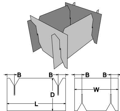
0. Standards\FEFCO Corrugated\0900 - Interior Fitments\FEFCO 0931 - Interior Compartment with Side Buffers
