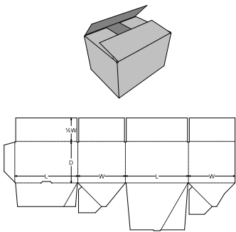
0. Standards\FEFCO Corrugated\0700 - Ready Glued - Self-Erecting Boxes\FEFCO 0701 - Full Crash Lock Auto Bottom, Regular Slotted Top - FCB/RSC
