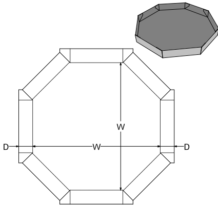
0. Standards\FEFCO Corrugated\0400 - Folder Type Boxes\FEFCO 0499 - Octagonal Glued Tray
