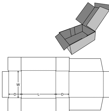
0. Standards\FEFCO Corrugated\0400 - Folder Type Boxes\FEFCO 0440 - Slitted Tray Full Depth Lid
