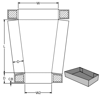
0. Standards\ECMA Folding Carton\Group D - Non-Long Seam Glued, Non-Rect. Surface\ D20.20.20.00 - Trapezium Single Walled Carton D2010
