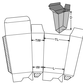
0. Standards\ECMA Folding Carton\Group C - Long Seam Glued, Non-Rect. Surface\ C20.20.60.20 - Tapered Carton, Crash Lock Base, Tuck to Front Top C2160
