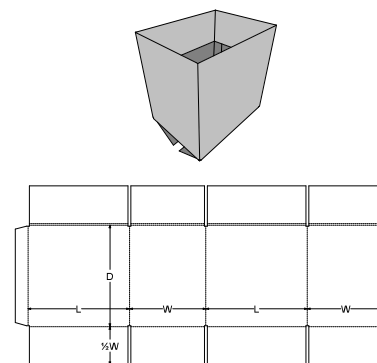
0. Standards\FEFCO Corrugated\0200 - Slotted Type Boxes\FEFCO 0214 - Roll Over Top Slotted Container - RSC
