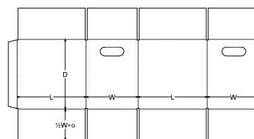
0. Standards\FEFCO Corrugated\0200 - Slotted Type Boxes\FEFCO 0202 HH - Overlap Slotted Container - HH
