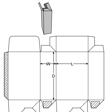
0. Standards\ECMA Folding Carton\Group A - Long Seam Glued, Rect. Surfaces\A60.45.00.01 - Sieve Proof Crash Lock Base A6045
