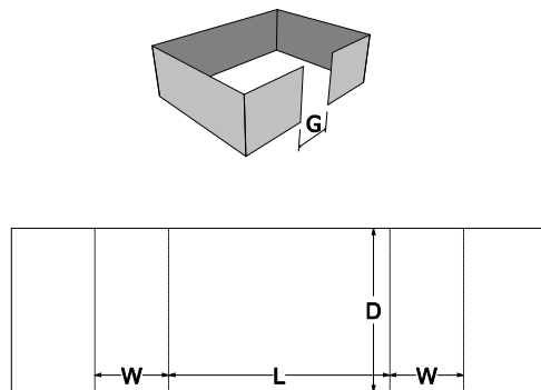
0. Standards\FEFCO Corrugated\0900 - Interior Fitments\FEFCO 0908 - Tube - Side Band - Centre Gap
