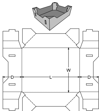
0. Standards\FEFCO Corrugated\0700 - Ready Glued - Self-Erecting Boxes\FEFCO 0771 - Style B - Reinforced Corner Tray
