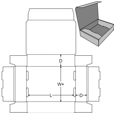
0. Standards\FEFCO Corrugated\0400 - Folder Type Boxes\FEFCO 0421 - Rolled End Tuck Tray
