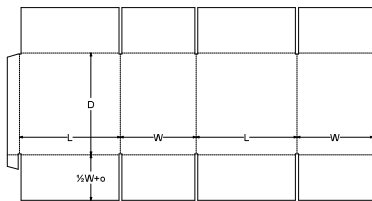
0. Standards\FEFCO Corrugated\0200 - Slotted Type Boxes\FEFCO 0202 EF - Overlap Slotted Container - Extended Flaps
