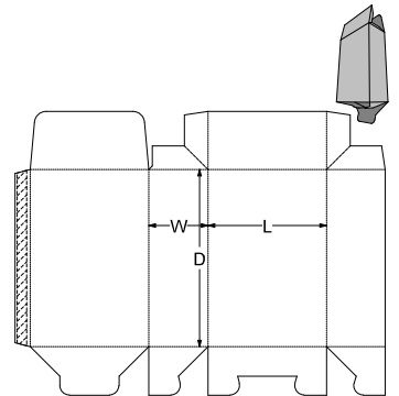
0. Standards\ECMA Folding Carton\Group A - Long Seam Glued, Rect. Surfaces\A55.45.01.01 - Sieve Proof Snap Lock Base A5545
