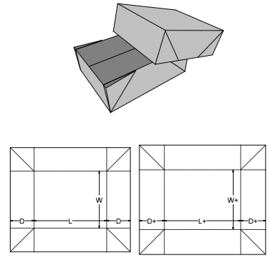
0. Standards\FEFCO Corrugated\0300 - Telescope Type Box\FEFCO 0309 - Webbed Corner Tray and Lid
