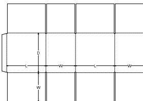
0. Standards\FEFCO Corrugated\0200 - Slotted Type Boxes\FEFCO 0203 - Full Overlap Slotted Container - FOL
