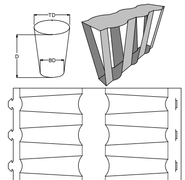
0. Standards\ECMA Folding Carton\Group E - Product Related or Integrated\E10.21.00.00 - Non-Glued Wrap E1021
