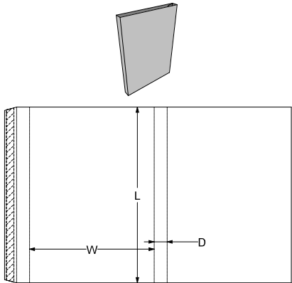
0. Standards\CD & DVD\DVD Slip Case - DVD Slip Case
