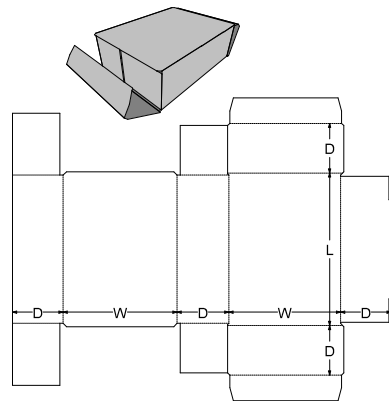
0. Standards\FEFCO Corrugated\0400 - Folder Type Boxes\FEFCO 0447 - Unglued End Tuck
