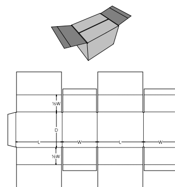
0. Standards\FEFCO Corrugated\0200 - Slotted Type Boxes\FEFCO 0229 - All Flaps Meet, Centre Partition
