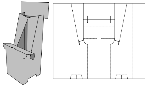
0. Standards\Display\2. Floor Standing Units\ Display Base - Centre Joint - Display Base - Centre Joint
