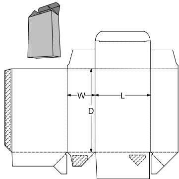
0. Standards\ECMA Folding Carton\Group A - Long Seam Glued, Rect. Surfaces\A61.20.01.03 - Tuck to Back Full Crash Lock Base A6120 Style A
