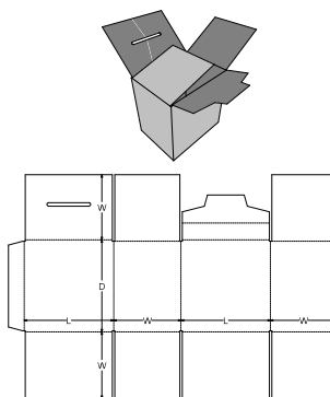
0. Standards\FEFCO Corrugated\0200 - Slotted Type Boxes\FEFCO 0218 - Recloseable Top, Full Overlapping Slotted Base - FOL
