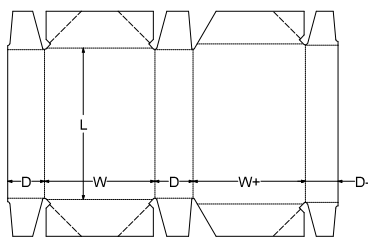
0. Standards\FEFCO Corrugated\0700 - Ready Glued - Self-Erecting Boxes\FEFCO 0760 - Style B - 6 Point Glued Tray with Cover
