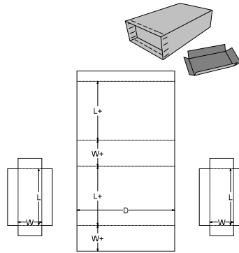
0. Standards\FEFCO Corrugated\0600 - Rigid Type Boxes - Bliss Boxes\FEFCO 0616 - Wrap with Internal Buffer End Caps
