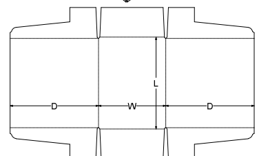
0. Standards\FEFCO Corrugated\0400 - Folder Type Boxes\FEFCO 0460 - High Wall Tray - Display Tray
