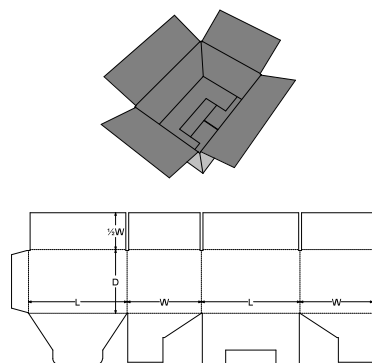
0. Standards\FEFCO Corrugated\0200 - Slotted Type Boxes\FEFCO 0216 - Regular Slotted Top, Envelope Base - RSC
