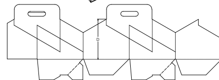
0. Standards\FEFCO Corrugated\0700 - Ready Glued - Self-Erecting Boxes\FEFCO 0717 - Style B - Crash Lock Base Auto Bottom, Bottle Carrier - CLB
