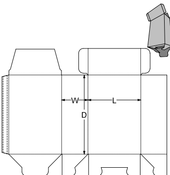
0. Standards\ECMA Folding Carton\Group A - Long Seam Glued, Rect. Surfaces\A55.40.01.03 - Side Tuck Snap Lock Base A5540
