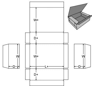
0. Standards\FEFCO Corrugated\0600 - Rigid Type Boxes - Bliss Boxes\FEFCO 0602 - Bliss Box Tuck
