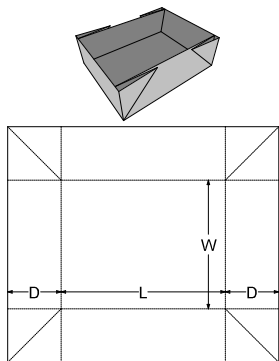
0. Standards\FEFCO Corrugated\0400 - Folder Type Boxes\FEFCO 0449 - Infold Tray Webbed Corners
