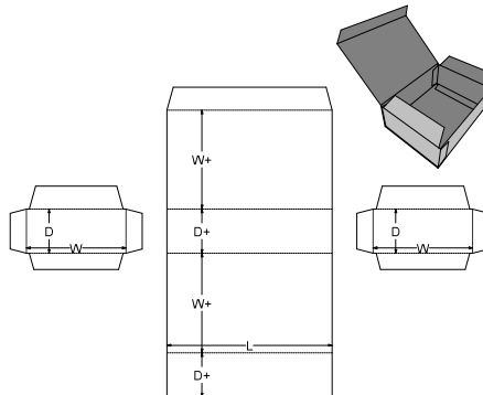
0. Standards\FEFCO Corrugated\0600 - Rigid Type Boxes - Bliss Boxes\FEFCO 0608 - Tuck Wrap with Internal End Caps
