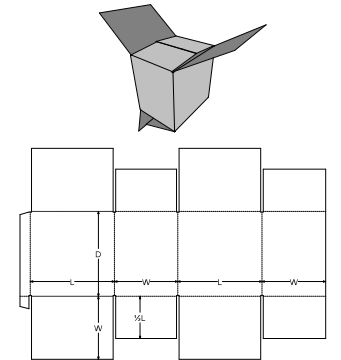
0. Standards\FEFCO Corrugated\0200 - Slotted Type Boxes\FEFCO 0206 EF - Overlap Sides, End Flaps Meet - SFF EFM
