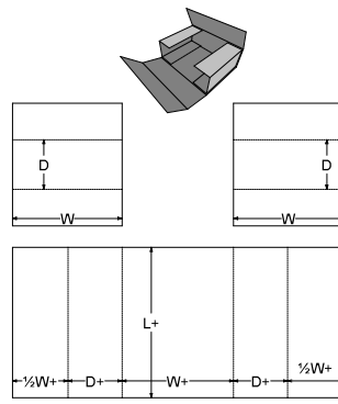
0. Standards\FEFCO Corrugated\0400 - Folder Type Boxes\FEFCO 0405 - Five Panel Wrap with End Caps
