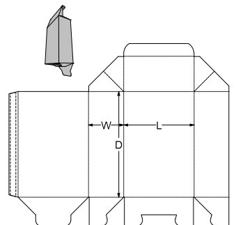
0. Standards\ECMA Folding Carton\Group A - Long Seam Glued, Rect. Surfaces\A55.20.01.03.99 (Webbed Tuck) - Webbed Tuck Snap Lock Base A5599
