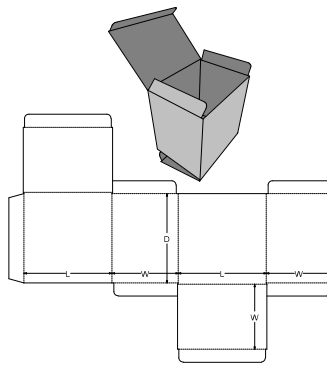
0. Standards\FEFCO Corrugated\0200 - Slotted Type Boxes\FEFCO 0211 - Reverse Tuck End, Tuck to Front Top, Tuck to Back Base
