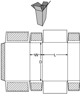
0. Standards\ECMA Folding Carton\Group A - Long Seam Glued, Rect. Surfaces\A11.11.03.03 (Bradman Lake End Load Skillet) - Bradman Lake End Load Skillet
