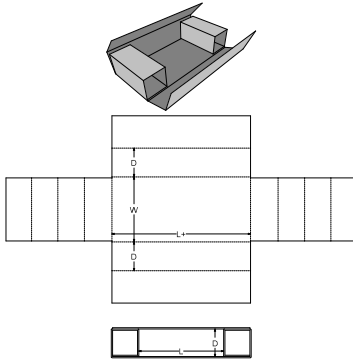
0. Standards\FEFCO Corrugated\0400 - Folder Type Boxes\FEFCO 0403 - One Piece Folder Buffer Ends - Air Cell
