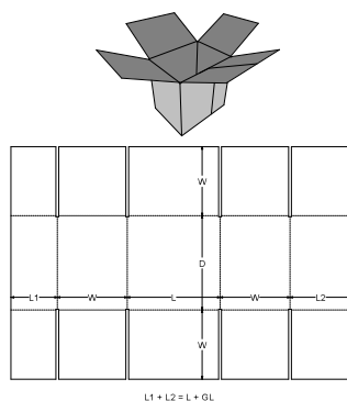
0. Standards\FEFCO Corrugated\0200 - Slotted Type Boxes\FEFCO 0230 - Full Overlapping Container, Centre Seam on Sides
