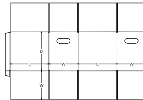
0. Standards\FEFCO Corrugated\0200 - Slotted Type Boxes\FEFCO 0203 EH - Full Overlap Slotted Container - FOL
