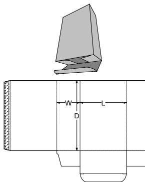
0. Standards\ECMA Folding Carton\Group A - Long Seam Glued, Rect. Surfaces\A20.01.03.00 - Tuck to Back - Open Top A2001
