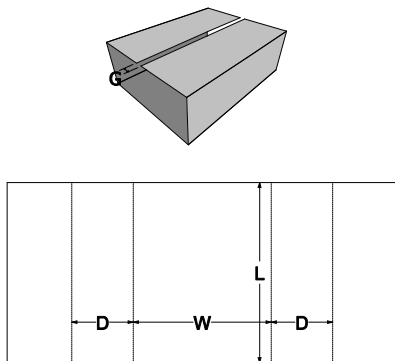
0. Standards\FEFCO Corrugated\0900 - Interior Fitments\FEFCO 0910 - Tube - Over Side Band - Centre Gap
