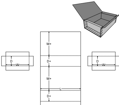
0. Standards\FEFCO Corrugated\0600 - Rigid Type Boxes - Bliss Boxes\FEFCO 0610 - Wrap with Internal Buffer End Caps
