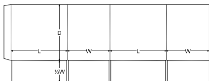
0. Standards\FEFCO Corrugated\0200 - Slotted Type Boxes\FEFCO 0200 - Half Slotted Container - HSC
