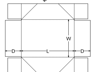
0. Standards\FEFCO Corrugated\0400 - Folder Type Boxes\FEFCO 0450 - Outfold Tray, End Slots
