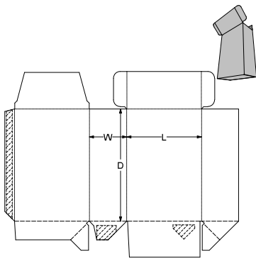
0. Standards\ECMA Folding Carton\Group A - Long Seam Glued, Rect. Surfaces\A61.40.01.03 - Side Tuck Full Crash Lock Base A6140
