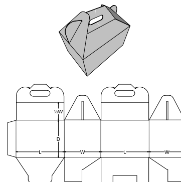
0. Standards\FEFCO Corrugated\0200 - Slotted Type Boxes\FEFCO 0217 - Carry Handle Top, Envelope Base
