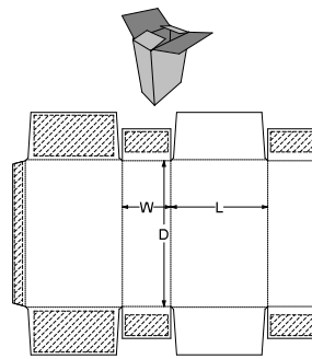
0. Standards\ECMA Folding Carton\Group A - Long Seam Glued, Rect. Surfaces\A11.11.03.03 (Jacob White End Load Skillet) - Jacob White End Load Skillet
