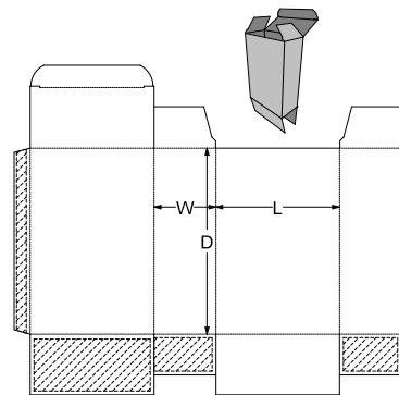
0. Standards\ECMA Folding Carton\Group A - Long Seam Glued, Rect. Surfaces\A11.20.03.01 - Tuck to Front Standard Skillet A1020
