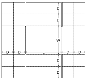
0. Standards\FEFCO Corrugated\0400 - Folder Type Boxes\FEFCO 0456 - Full Reinforced Tray
