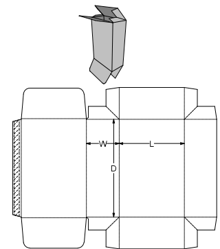
0. Standards\ECMA Folding Carton\Group A - Long Seam Glued, Rect. Surfaces\A45.45.01.01 - Sieve Proof Top and Base A4545
