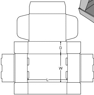
0. Standards\FEFCO Corrugated\0400 - Folder Type Boxes\FEFCO 0429 - Rolled End Tuck Tray with Dust Flaps
