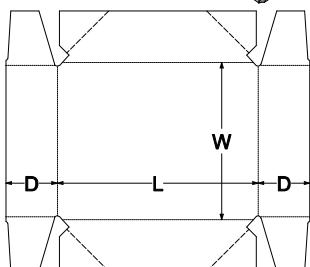
0. Standards\FEFCO Corrugated\0400 - Folder Type Boxes\FEFCO 0451 - Style B - Infold Tray
