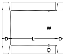
0. Standards\FEFCO Corrugated\0400 - Folder Type Boxes\FEFCO 0452 - Style B - Diecut Side Slotted Tray
