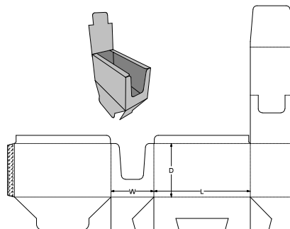
0. Standards\ECMA Folding Carton\Group A - Long Seam Glued, Rect. Surfaces\A55.20.01.04.35 (Display Outer) - Display Outer Snap Lock Base FC0603
