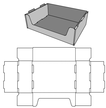
0. Standards\Display\3. Trays, Shelf Ready and Fillers\Stackable Rolled End Tray - Rolled End Tray (Fefco 0422)
