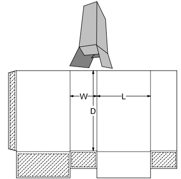
0. Standards\ECMA Folding Carton\Group A - Long Seam Glued, Rect. Surfaces\A11.01.03.00 - Open Ended Square Flap Skillet
