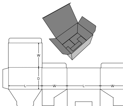
0. Standards\FEFCO Corrugated\0200 - Slotted Type Boxes\FEFCO 0215 - Tuck to Front Top, Envelope Base
