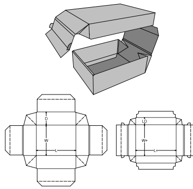
0. Standards\FEFCO Corrugated\0300 - Telescope Type Box\FEFCO 0323 - Self Locking Webbed Tray and Lid
