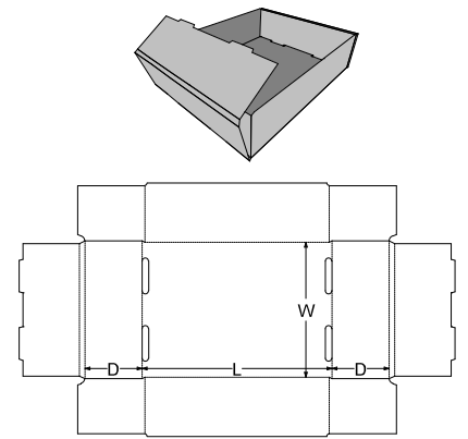
0. Standards\FEFCO Corrugated\0400 - Folder Type Boxes\FEFCO 0422 - Rolled End Tray
