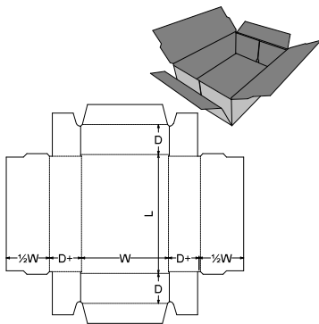
0. Standards\FEFCO Corrugated\0400 - Folder Type Boxes\FEFCO 0415 - One Piece Taped Folder with Dust Flaps - OPF
