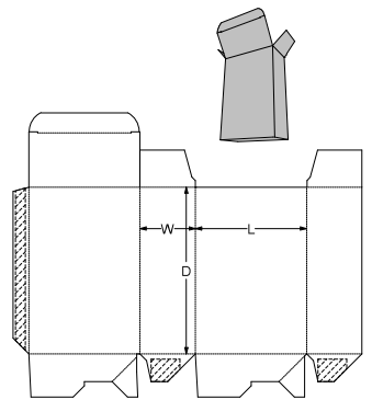
0. Standards\ECMA Folding Carton\Group A - Long Seam Glued, Rect. Surfaces\A60.20.00.01 - Tuck to Front Crash Lock Base A6020
