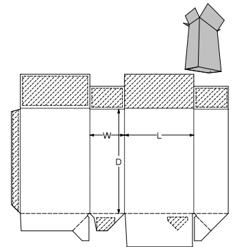
0. Standards\ECMA Folding Carton\Group A - Long Seam Glued, Rect. Surfaces\A61.11.01.03 - Square Skillet Full Crash Lock Base A6110
