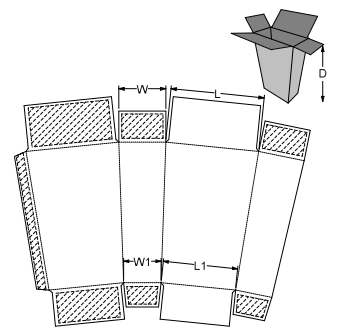
0. Standards\ECMA Folding Carton\Group C - Long Seam Glued, Non-Rect. Surface\ C20.20.10.10 - Tapered Skillet Top and Bottom C2110
