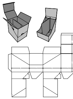
0. Standards\FEFCO Corrugated\0700 - Ready Glued - Self-Erecting Boxes\FEFCO 0716 - Crash Lock Base Auto Bottom with Divider, Tuck Display Centre Divider - CLB/TF
