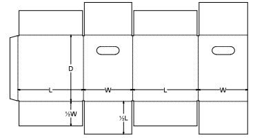
0. Standards\FEFCO Corrugated\0200 - Slotted Type Boxes\FEFCO 0204 HH - All Flaps Meet Slotted Container - AFM - CSSC HH
