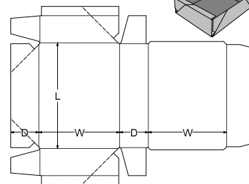
0. Standards\FEFCO Corrugated\0700 - Ready Glued - Self-Erecting Boxes\FEFCO 0747 - 4 Point Side Glued Tuck Tray
