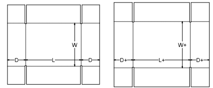
0. Standards\FEFCO Corrugated\0300 - Telescope Type Box\FEFCO 0300 - Side Slotted Tray and Lid
