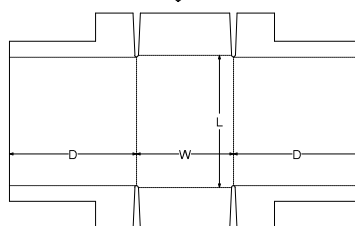
0. Standards\FEFCO Corrugated\0400 - Folder Type Boxes\FEFCO 0460 - Style B - High Wall Tray - Display Tray
