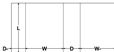
0. Standards\FEFCO Corrugated\0900 - Interior Fitments\FEFCO 0906 - Tube - Over Side - Side Gap
