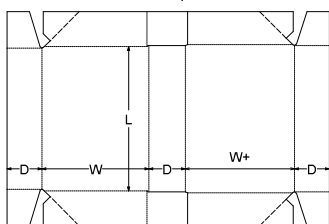
0. Standards\FEFCO Corrugated\0700 - Ready Glued - Self-Erecting Boxes\FEFCO 0759 - 4 Point Glued Tray with Lid
