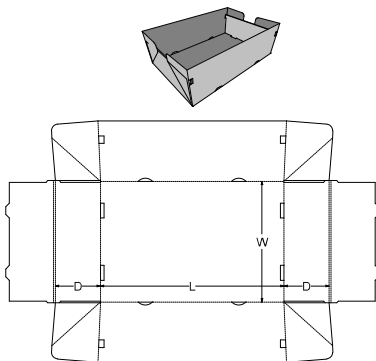
0. Standards\FEFCO Corrugated\0700 - Ready Glued - Self-Erecting Boxes\FEFCO 0772 - Infold Locking Tray
