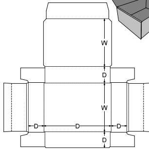
0. Standards\FEFCO Corrugated\0400 - Folder Type Boxes\FEFCO 0428 - Rolled End Slot-less Tuck Tray
