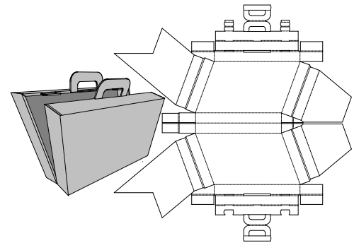
0. Standards\Display\5. Carry Cases\Carry Case (Rhombus)
