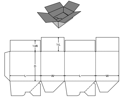
0. Standards\FEFCO Corrugated\0700 - Ready Glued - Self-Erecting Boxes\FEFCO 0712 - Style B - Crash Lock Base Auto Bottom, All Flaps Meet Top - CLB/AFM
