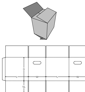
0. Standards\FEFCO Corrugated\0200 - Slotted Type Boxes\FEFCO 0205 HH - End Flaps Meet Slotted Container - CSO EFM HH
