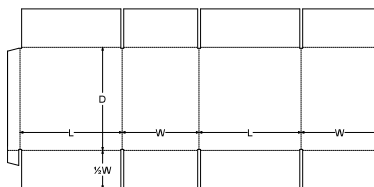
0. Standards\FEFCO Corrugated\0200 - Slotted Type Boxes\FEFCO 0201 EF - Regular Slotted Container Extended Flaps - HSC EF
