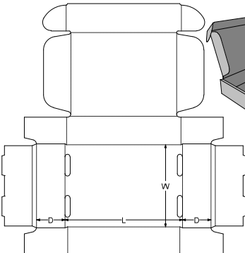
0. Standards\FEFCO Corrugated\0400 - Folder Type Boxes\FEFCO 0427 - Rolled End Tuck Tray, Dust Flaps and Cherry Locks
