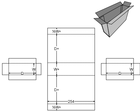
0. Standards\FEFCO Corrugated\0600 - Rigid Type Boxes - Bliss Boxes\FEFCO 0620 - Wrap with Internal Side Caps
