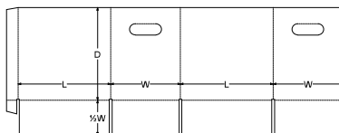
0. Standards\FEFCO Corrugated\0200 - Slotted Type Boxes\FEFCO 0200 EH - Half Slotted Container Extended Glue Flap Hand Holes - HSC EF HH
