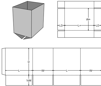
0. Standards\FEFCO Corrugated\0300 - Telescope Type Box\FEFCO 0312 - Half Slotted Container with Lid - HSC
