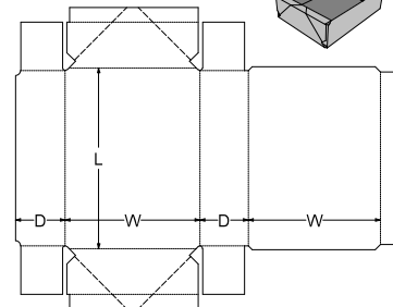
0. Standards\FEFCO Corrugated\0700 - Ready Glued - Self-Erecting Boxes\FEFCO 0748 - Style B - 4 Point Glued Tuck Tray
