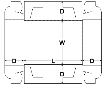
0. Standards\FEFCO Corrugated\0400 - Folder Type Boxes\FEFCO 0457 - Self Locking Tray
