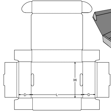
0. Standards\FEFCO Corrugated\0400 - Folder Type Boxes\FEFCO 0427 - Variation A - Rolled End Tuck Tray, Cherry Locks and No Dust Flaps
