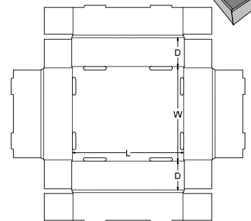
0. Standards\FEFCO Corrugated\0400 - Folder Type Boxes\FEFCO 0425 - Rolled 4 Sides Tray
