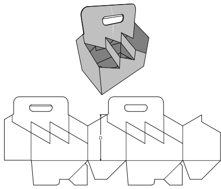
0. Standards\FEFCO Corrugated\0700 - Ready Glued - Self-Erecting Boxes\FEFCO 0717 - Crash Lock Base Auto Bottom, Bottle Carrier - CLB
