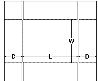
0. Standards\FEFCO Corrugated\0400 - Folder Type Boxes\FEFCO 0452 - Side Slotted Tray
