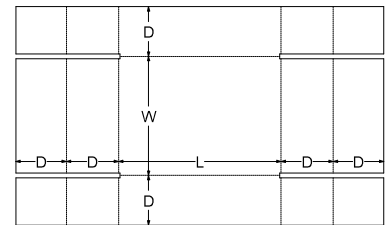
0. Standards\FEFCO Corrugated\0400 - Folder Type Boxes\FEFCO 0454 - Tray Folded Ends
