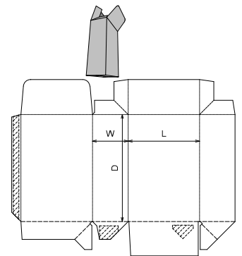
0. Standards\ECMA Folding Carton\Group A - Long Seam Glued, Rect. Surfaces\A61.45.01.01 - Sieve Proof Full Crash Lock Base A6145
