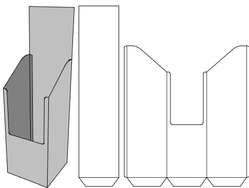
0. Standards\Display\2. Floor Standing Units\ Pallet Wrap - Turn Over Back w/Flange - Pallet Wrap - Turn Over Back w/Flange
