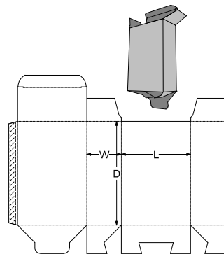
0. Standards\ECMA Folding Carton\Group A - Long Seam Glued, Rect. Surfaces\A55.20.01.01 - Tuck to Front Snap Lock Base A5520 Style B
