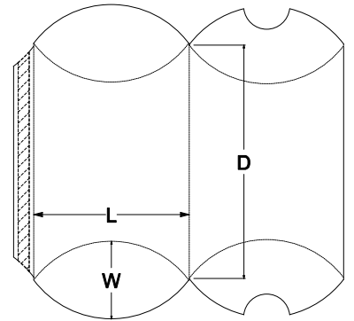
0. Standards\ECMA Folding Carton\Group F - Other Folding Carton Styles\F70.01.00.00 Style A - Pillow Pack F7001 Style A
