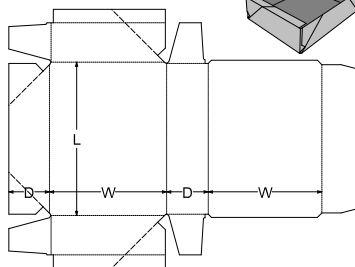
0. Standards\FEFCO Corrugated\0700 - Ready Glued - Self-Erecting Boxes\FEFCO 0747 - Style B - 4 Point Side Glued Tuck Tray
