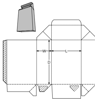
0. Standards\ECMA Folding Carton\Group A - Long Seam Glued, Rect. Surfaces\A61.20.01.03.99 (Webbed Tuck) - Webbed Tuck Full Crash Lock Base A6199
