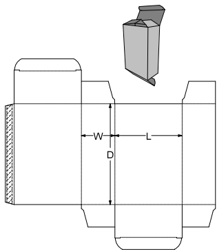
0. Standards\ECMA Folding Carton\Group A - Long Seam Glued, Rect. Surfaces\A20.20.03.01 - Reverse Tuck End A2120
