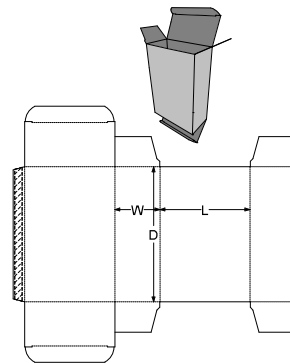
0. Standards\ECMA Folding Carton\Group A - Long Seam Glued, Rect. Surfaces\A20.20.01.01 - Aerotuck to Back A2320
