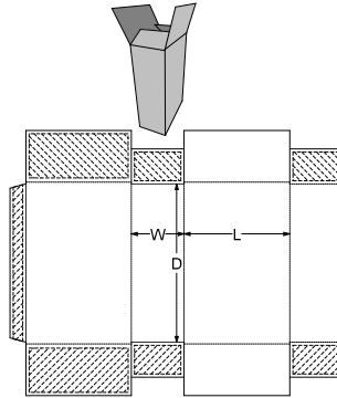
0. Standards\ECMA Folding Carton\Group A - Long Seam Glued, Rect. Surfaces\A11.11.03.03 - Square Flap Skillet A1010
