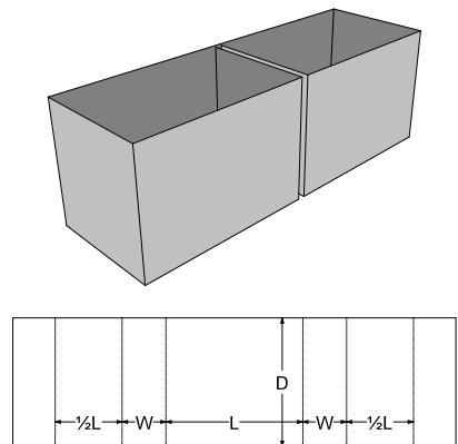
0. Standards\FEFCO Corrugated\0900 - Interior Fitments\FEFCO 0920 - Interior Buffer
