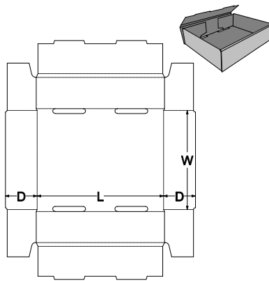
0. Standards\FEFCO Corrugated\0400 - Folder Type Boxes\FEFCO 0423 - Rolled Side Tray
