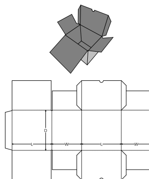
0. Standards\FEFCO Corrugated\0200 - Slotted Type Boxes\FEFCO 0227 - Slotted Tuck Top and Base
