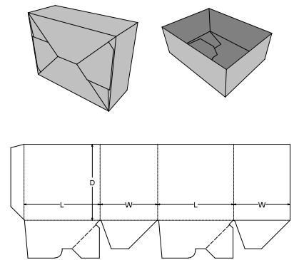
0. Standards\FEFCO Corrugated\0700 - Ready Glued - Self-Erecting Boxes\FEFCO 0700 - Crash Lock Auto Bottom, Open Top - CLB/OT
