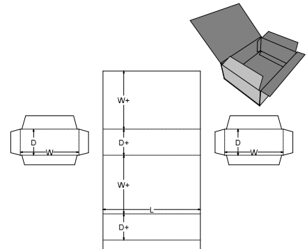
0. Standards\FEFCO Corrugated\0600 - Rigid Type Boxes - Bliss Boxes\FEFCO 0607 - Wrap with Internal End Caps
