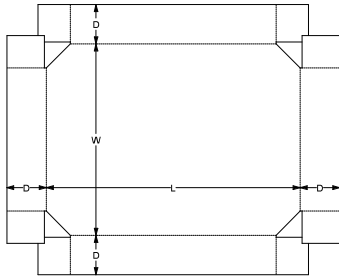
0. Standards\FEFCO Corrugated\0400 - Folder Type Boxes\FEFCO 0459 - Can Tray
