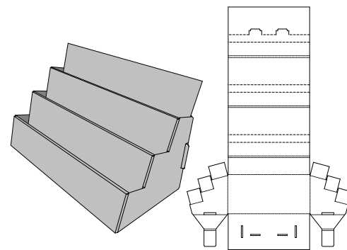
0. Standards\Display\1. Counter Top Units\Multi-Tier Shelf - Multi-Tier Shelf
