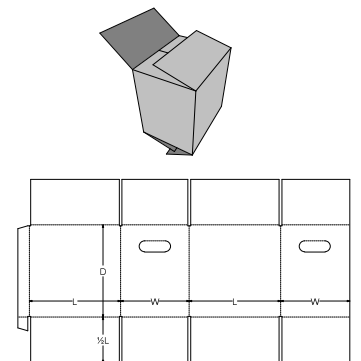
0. Standards\FEFCO Corrugated\0200 - Slotted Type Boxes\FEFCO 0205 EH - End Flaps Meet Slotted Container - CSO EFM
