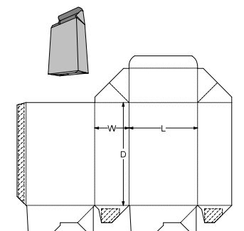
0. Standards\ECMA Folding Carton\Group A - Long Seam Glued, Rect. Surfaces\A60.20.00.03.99 (Webbed Tuck) - Webbed Tuck Crash Lock Base A6099
