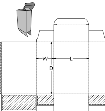
0. Standards\ECMA Folding Carton\Group A - Long Seam Glued, Rect. Surfaces\A11.20.03.03 - Tuck to Back Standard Skillet A1020
