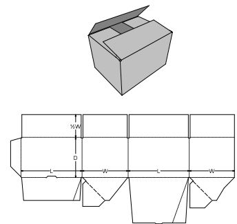
0. Standards\FEFCO Corrugated\0700 - Ready Glued - Self-Erecting Boxes\FEFCO 0701 - Style B - Full Crash Lock Auto Bottom, Regular Slotted Top - FCB/RSC
