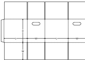
0. Standards\FEFCO Corrugated\0200 - Slotted Type Boxes\FEFCO 0203 HH - Full Overlap Slotted Container - FOL
