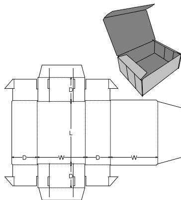
0. Standards\FEFCO Corrugated\0400 - Folder Type Boxes\FEFCO 0445 - End Lock Tuck Tray
