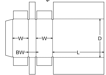
0. Standards\FEFCO Corrugated\0600 - Rigid Type Boxes - Bliss Boxes\FEFCO 0621 - 2 Piece Buffer Ends
