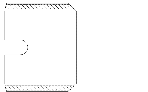
0. Standards\CD & DVD\CD Single Fold Sleeve - Style B - CD Single Fold Sleeve - Glue to back
