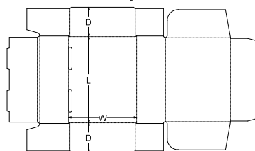
0. Standards\FEFCO Corrugated\0400 - Folder Type Boxes\FEFCO 0426 - Rolled Side Tuck Tray with Dust Flaps - Pizza Box
