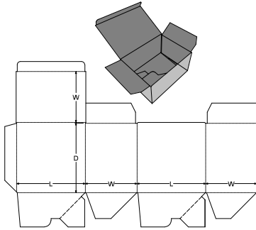
0. Standards\FEFCO Corrugated\0700 - Ready Glued - Self-Erecting Boxes\FEFCO 0713 - Style B - Crash Lock Base Auto Bottom, Tuck to Front Top - CLB/TF
