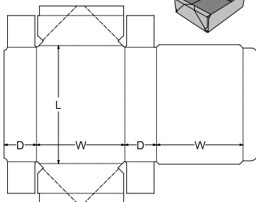
0. Standards\FEFCO Corrugated\0700 - Ready Glued - Self-Erecting Boxes\FEFCO 0748 - 4 Point Glued Tuck Tray
