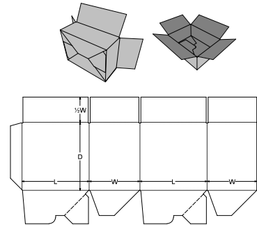
0. Standards\FEFCO Corrugated\0700 - Ready Glued - Self-Erecting Boxes\FEFCO 0711 - Crash Lock Auto Bottom, Regular Slotted Top - CLB/RSC
