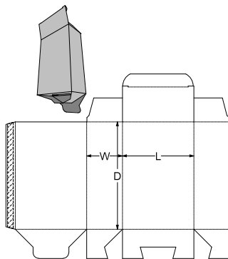
0. Standards\ECMA Folding Carton\Group A - Long Seam Glued, Rect. Surfaces\A55.20.01.03 - Tuck to Back Snap Lock Base A5520 Style A
