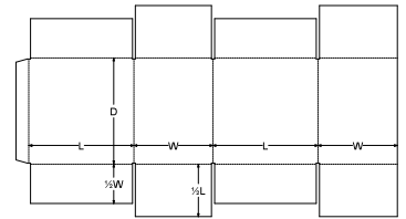
0. Standards\FEFCO Corrugated\0200 - Slotted Type Boxes\FEFCO 0204 - All Flaps Meet Slotted Container - AFM - CSSC
