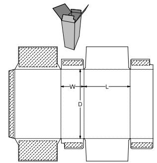
0. Standards\ECMA Folding Carton\Group A - Long Seam Glued, Rect. Surfaces\A11.11.03.03 (Captain End Load Skillet) - Captain End Load Skillet
