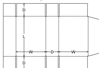
0. Standards\FEFCO Corrugated\0400 - Folder Type Boxes\FEFCO 0410 - Five Panel Folder - FPF
