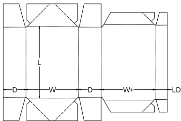
0. Standards\FEFCO Corrugated\0700 - Ready Glued - Self-Erecting Boxes\FEFCO 0761 - 6 Point Glued Tray with Cover
