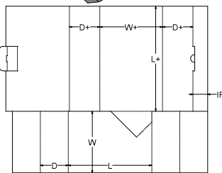
0. Standards\FEFCO Corrugated\0400 - Folder Type Boxes\FEFCO 0473 - Twist Folder
