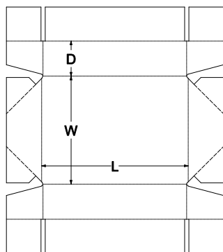
0. Standards\FEFCO Corrugated\0700 - Ready Glued - Self-Erecting Boxes\FEFCO 0718 - Style B - 4 Point Glued Tray
