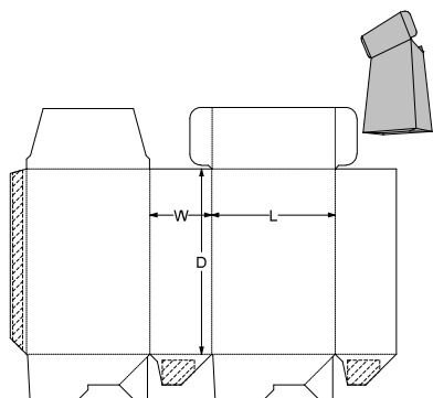
0. Standards\ECMA Folding Carton\Group A - Long Seam Glued, Rect. Surfaces\A60.40.00.03 - Side Tuck Crash Lock Base A6040
