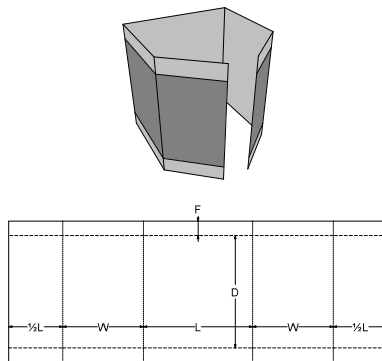
0. Standards\FEFCO Corrugated\0900 - Interior Fitments\FEFCO 0913 - Fold Over Centre Seam Insert
