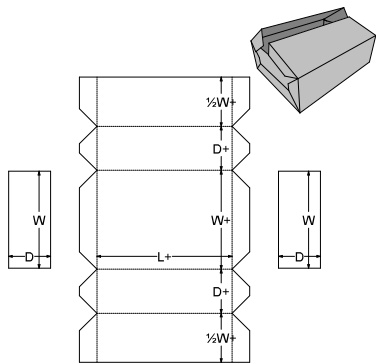
0. Standards\FEFCO Corrugated\0600 - Rigid Type Boxes - Bliss Boxes\FEFCO 0606 - Bliss Box Centre Seam
