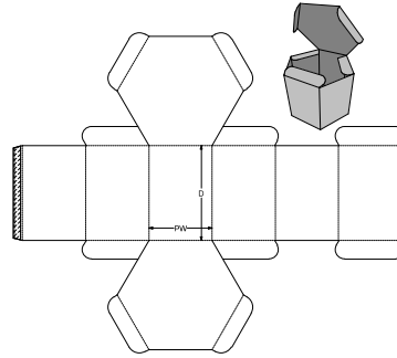
0. Standards\ECMA Folding Carton\Group C - Long Seam Glued, Non-Rect. Surface\ C10.40.20.20 - Hexagonal Same Panel Tuck C4020
