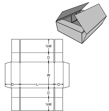
0. Standards\FEFCO Corrugated\0400 - Folder Type Boxes\FEFCO 0412 - Courier Pack, Diecut Centre Taped
