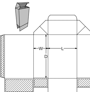
0. Standards\ECMA Folding Carton\Group A - Long Seam Glued, Rect. Surfaces\A11.20.03.03.99 (Webbed Tuck) - Webbed Tuck Square Flap Skillet A1099
