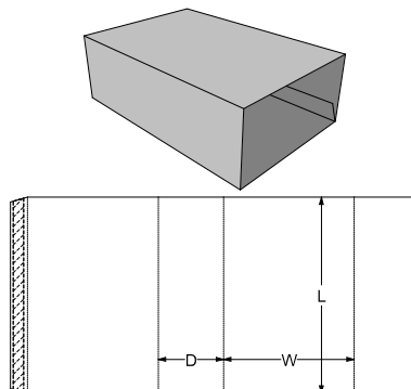
0. Standards\ECMA Folding Carton\Group E - Product Related or Integrated\E30.20.00.00 - Sleeve With/Without Thumb Cuts E3120
