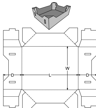
0. Standards\FEFCO Corrugated\0700 - Ready Glued - Self-Erecting Boxes\FEFCO 0771 - Reinforced Corner Tray
