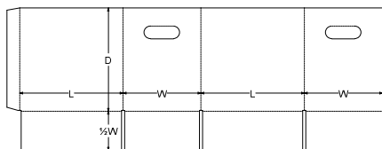
0. Standards\FEFCO Corrugated\0200 - Slotted Type Boxes\FEFCO 0200 HH - Half Slotted Container Hand Holes - HSC HH
