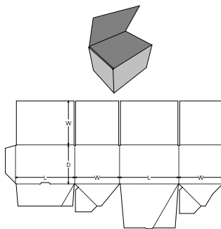
0. Standards\FEFCO Corrugated\0700 - Ready Glued - Self-Erecting Boxes\FEFCO 0703 - Full Crash Lock Auto Bottom, Full Overlapping Top - FCB/FOL
